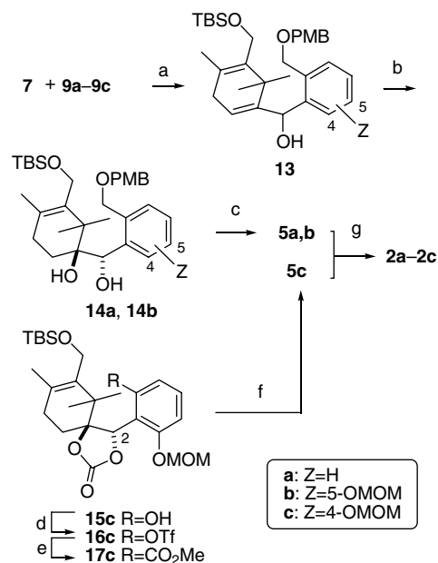
Scheme 2. The synthesis of nine-membered ethers 2 . Reagents and conditions: (a) THF, -78^\circ C , 13a (83%); 13b (53%); 13c (64%); (b) (i) VO(acac)_2 , t -BuOOH, benzene; (ii) LiAlH_4 , ether, reflux; (iii) TBSCl, imidazole, CH_2Cl_2 , 14a (88%); 14b (72%); (c) (i) carbonyldiimidazole, CH_3CN , reflux; (ii) TBAF, THF; (iii) MsCl , LiCl , NEt_3 , THF, CH_2Cl_2 ; (iv) DDQ, CH_2Cl_2 , H_2O , 5a (69%); 5b (66%); (d) Tf_2O , NEt_3 , CH_2Cl_2 , 85%; (e) CO (15 atm), Pd(OAc)_2 , DPPP, NEt_3 , MeOH, THF, 80^\circ C , quant.; (f) (i) LiAlH_4 , ether; (ii) Ac_2O , NEt_3 , CH_2Cl_2 ; (iii) carbonyldiimidazole, CH_3CN , reflux (iv) TBAF, AcOH, THF; (v) MsCl , LiCl , NEt_3 , CH_2Cl_2 , THF; (vi) K_2CO_3 , MeOH, 5c (66%); (g) NaH, PhH, DC-18-crown-6, RT, 2a (66%); 2b (92%); 2c (64%).
