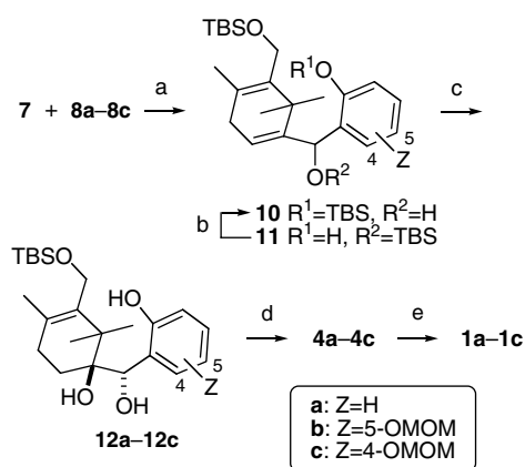
Scheme 1. The synthesis of eight-membered ethers 1 . Reagents and conditions: (a) THF, -78^\circ C ; (b) (i) K_2CO_3 , MeOH; (ii) TBSCl, imidazole, CH_2Cl_2 , 10a (89%); 10b (68%); 10c (61%); (c) (i) VO(acac)_2 , t -BuOOH, benzene; (ii) LiAlH_4 , ether, 12a (91%); 12b (93%); 12c (58%); (d) (i) TBSCl, imidazole, CH_2Cl_2 ; (ii) carbonyldiimidazole, CH_3CN , reflux; (iii) TBAF, THF, 4a (52%); 4b (94%); 4c (61%); (viii) PPh_3 , DEAD, THF, RT, 1a (85%); 1b (96%); 1c (65%).
